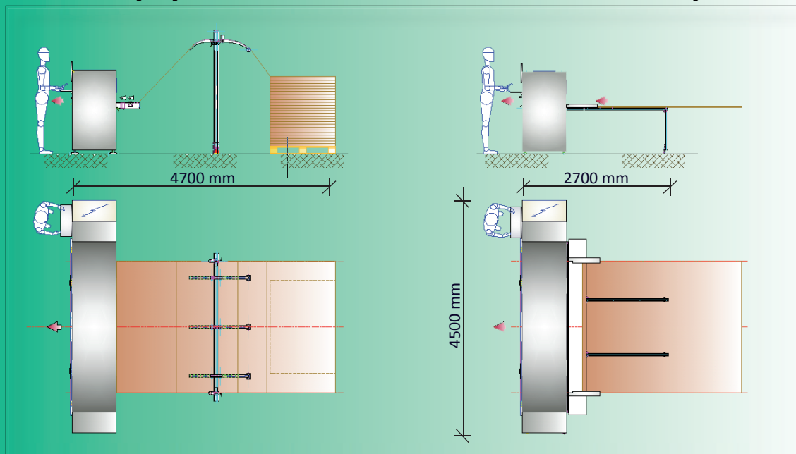
Machine with fan fold cardboard
